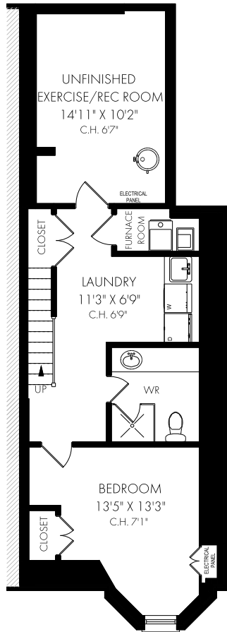
LOWER LEVEL - 717 SQUARE FEET
