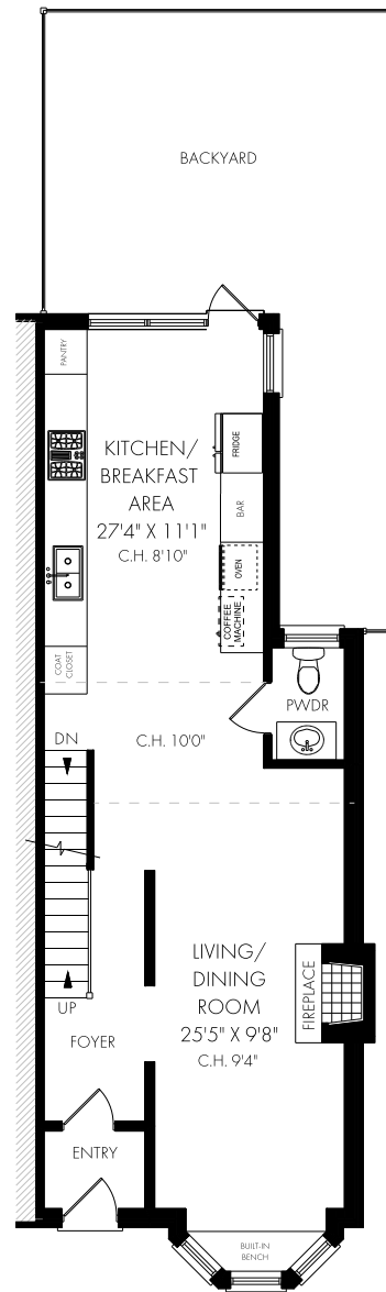
MAIN FLOOR - 717 SQUARE FEET
