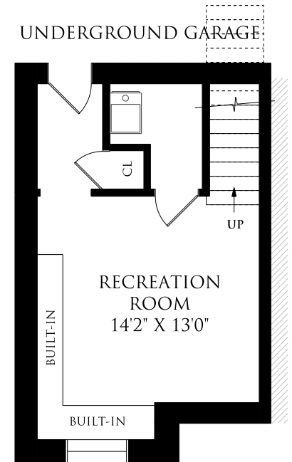
LOWER LEVEL 338 SQUARE FEET CEILING HEIGHT 7'10"
