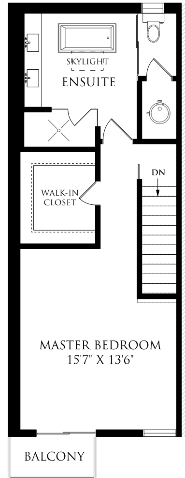
THIRD FLOOR 558 SQUARE FEET CEILING HEIGHT 9'0"
