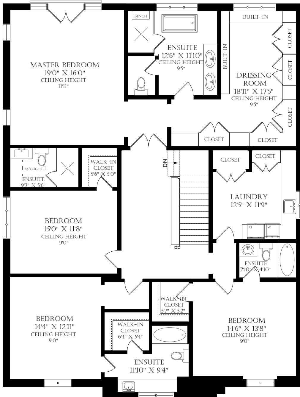
SECOND FLOOR 2286 SQUARE FEET
